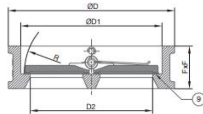
DN600 - DN800 SECTION A - A
