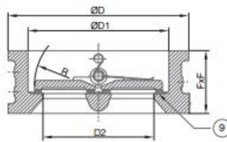
DN50 - DN500 SECTION A - A
