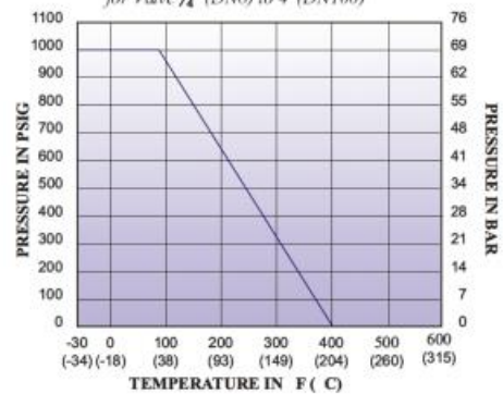
Pressure Vs. Temperature Chart for Valve V_4 (DN8) to 4" (DN100)
